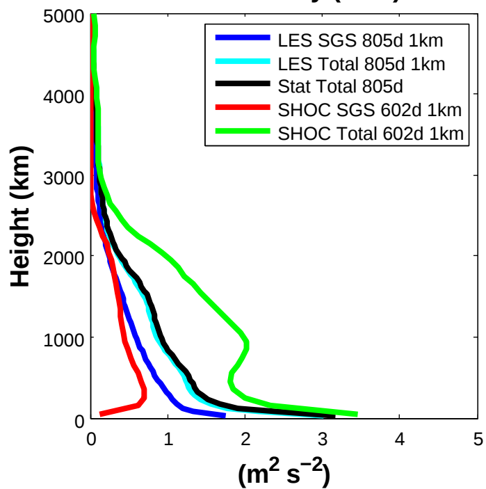
TKE Ice Only (1km)
