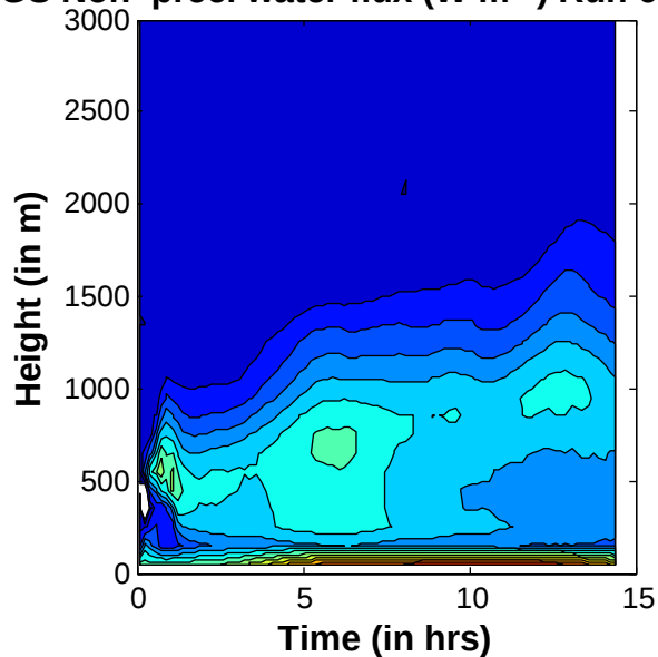
SGS Non-prec. water flux ( \text{W m}^{-2} ) Run 603d (.5km) SGS Non-prec. water flux ( \text{W m}^{-2} ) Run 805d (.1km)
