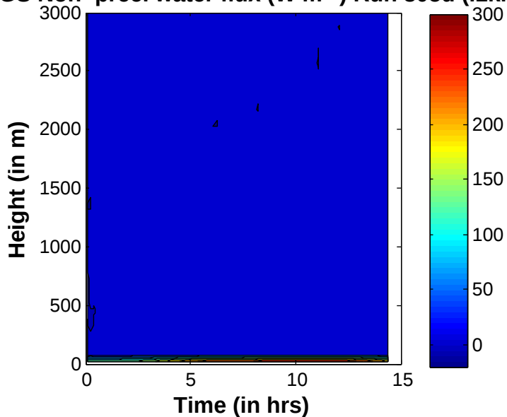
SGS Non-prec. water flux ( \text{W m}^{-2} ) Run 603d (.5km) SGS Non-prec. water flux ( \text{W m}^{-2} ) Run 805d (.1km)
