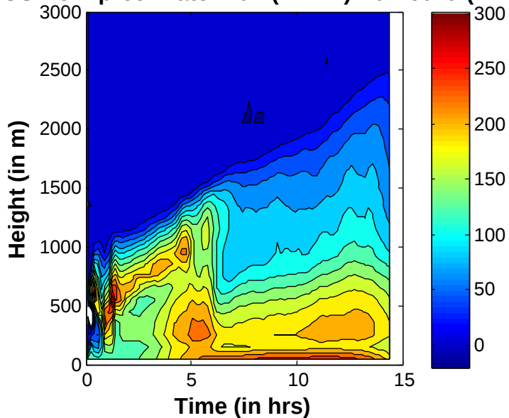
SGS Non-prec. water flux ( \text{W m}^{-2} ) Run 601d (3km) SGS Non-prec. water flux ( \text{W m}^{-2} ) Run 602d (1km)
