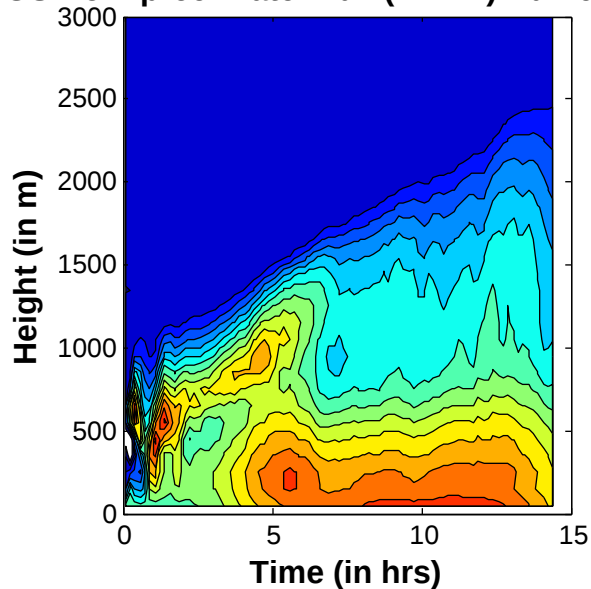
SGS Non-prec. water flux ( \text{W m}^{-2} ) Run 601d (3km) SGS Non-prec. water flux ( \text{W m}^{-2} ) Run 602d (1km)
