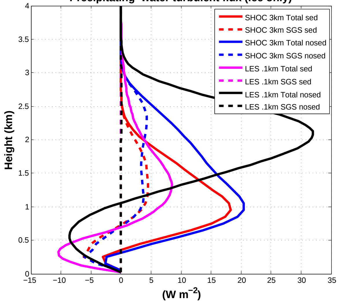
Precipitating-water turbulent flux (ice only)
