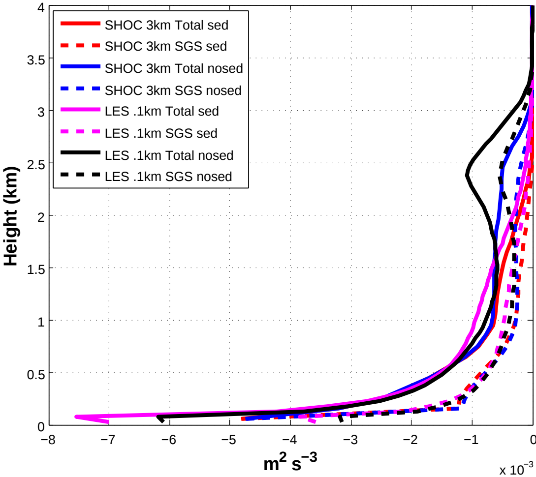
Dissipation terms of TKE (ice only)
