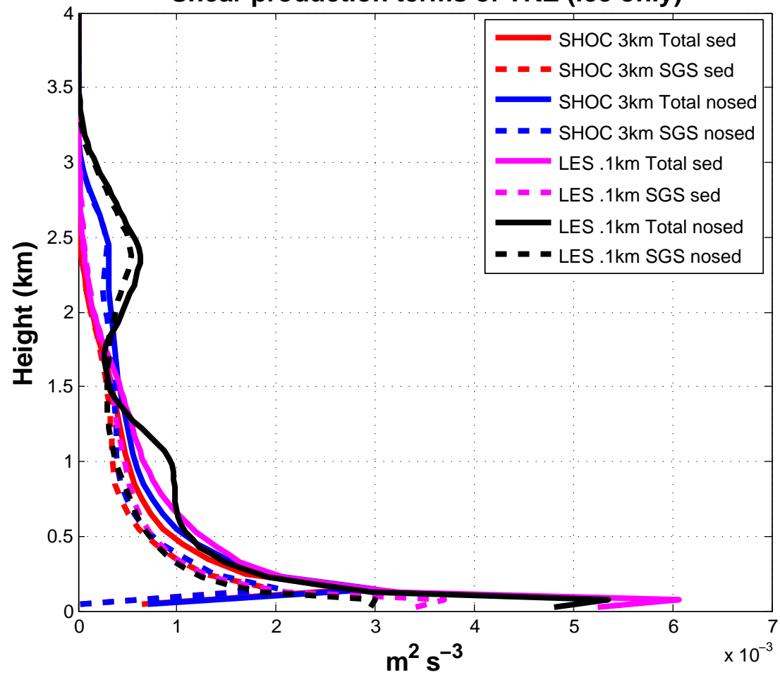
Shear production terms of TKE (ice only)
