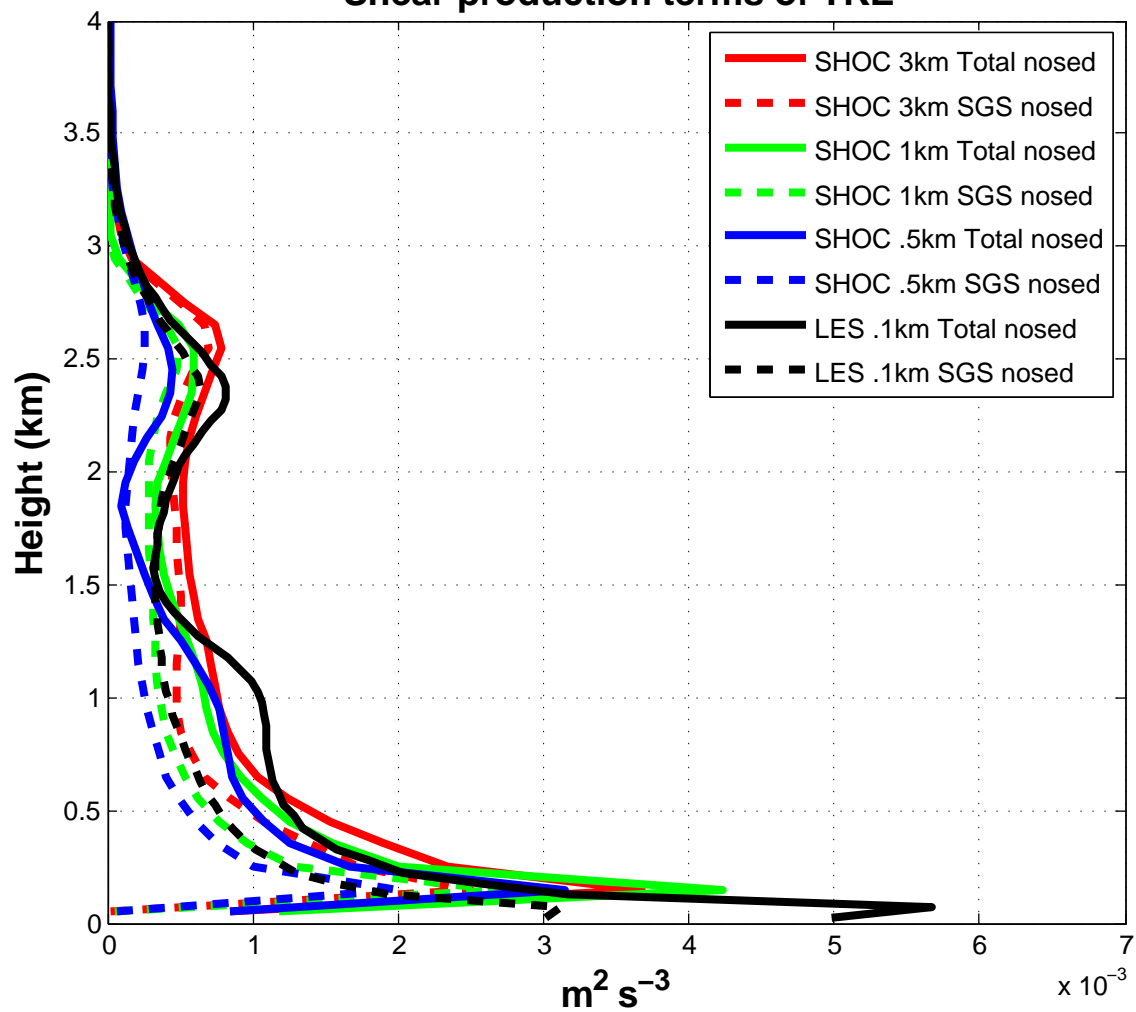
Shear production terms of TKE
