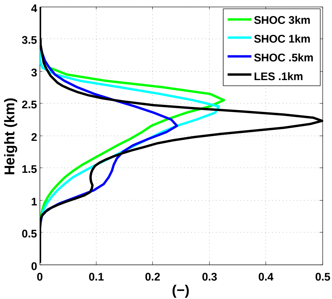
Cloud Fraction (No Sed.)
