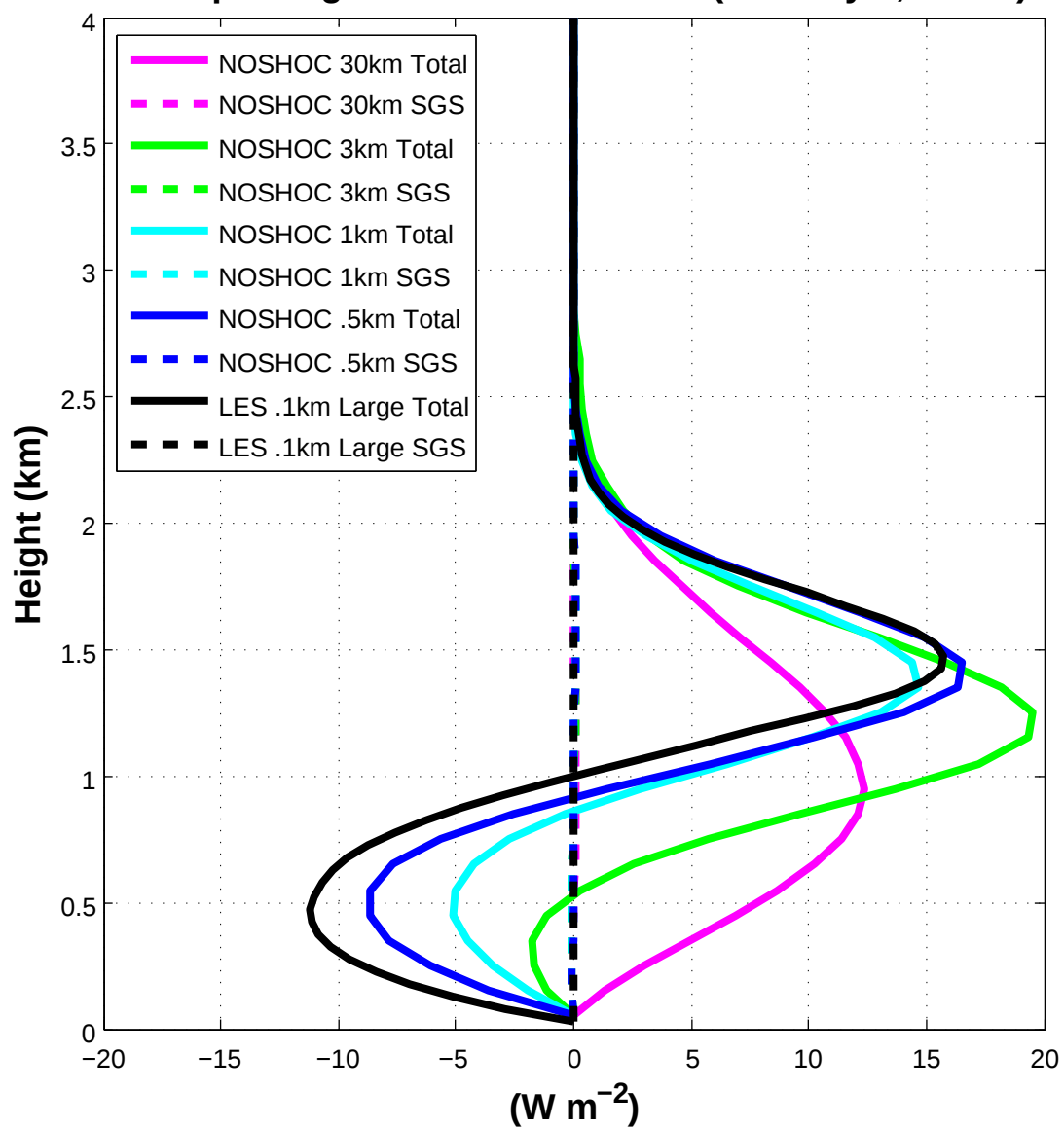
Precipitating-water turbulent flux (Full Phys., norad)
