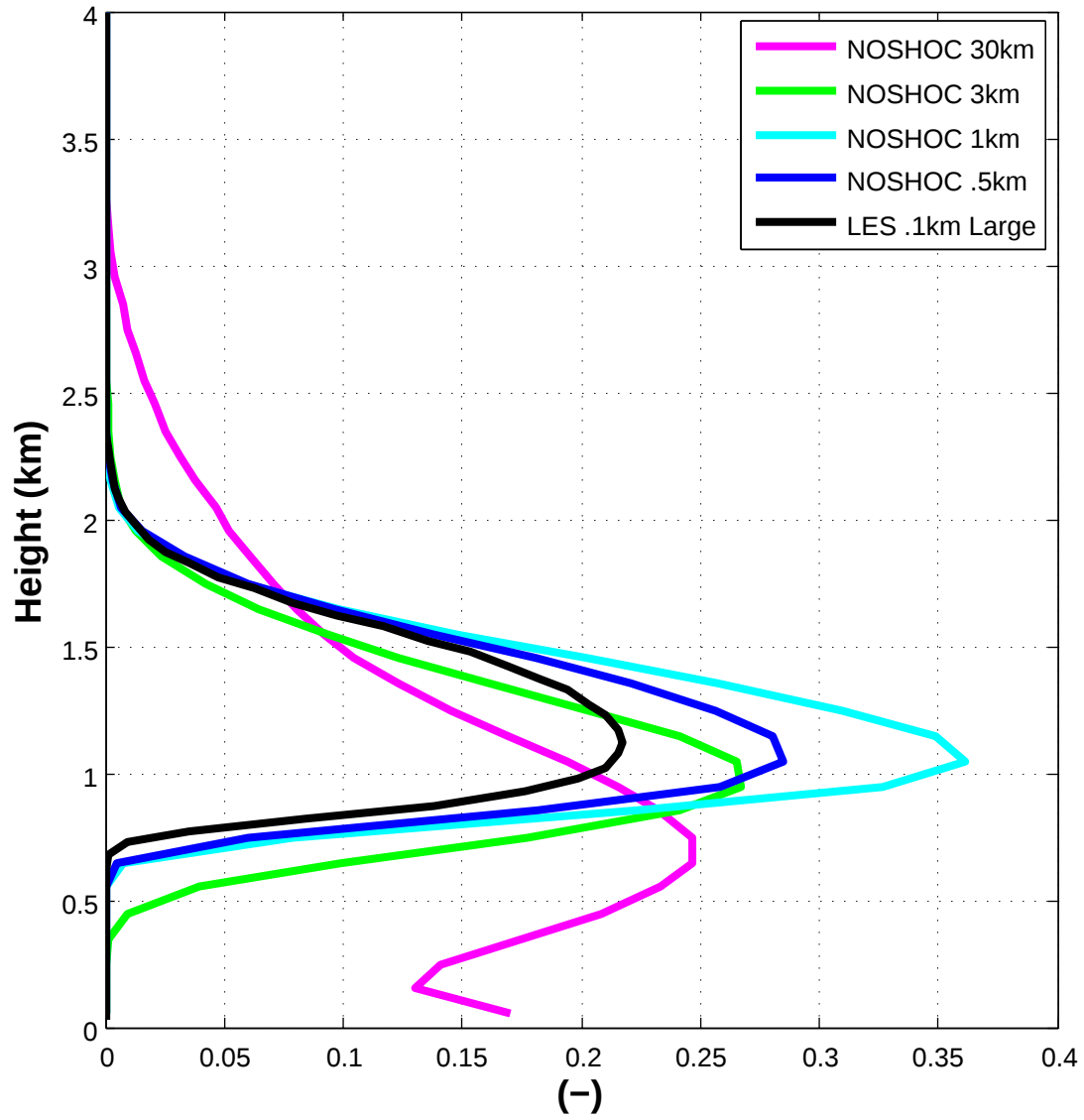
Cloud Fraction (Full Phys., norad)
