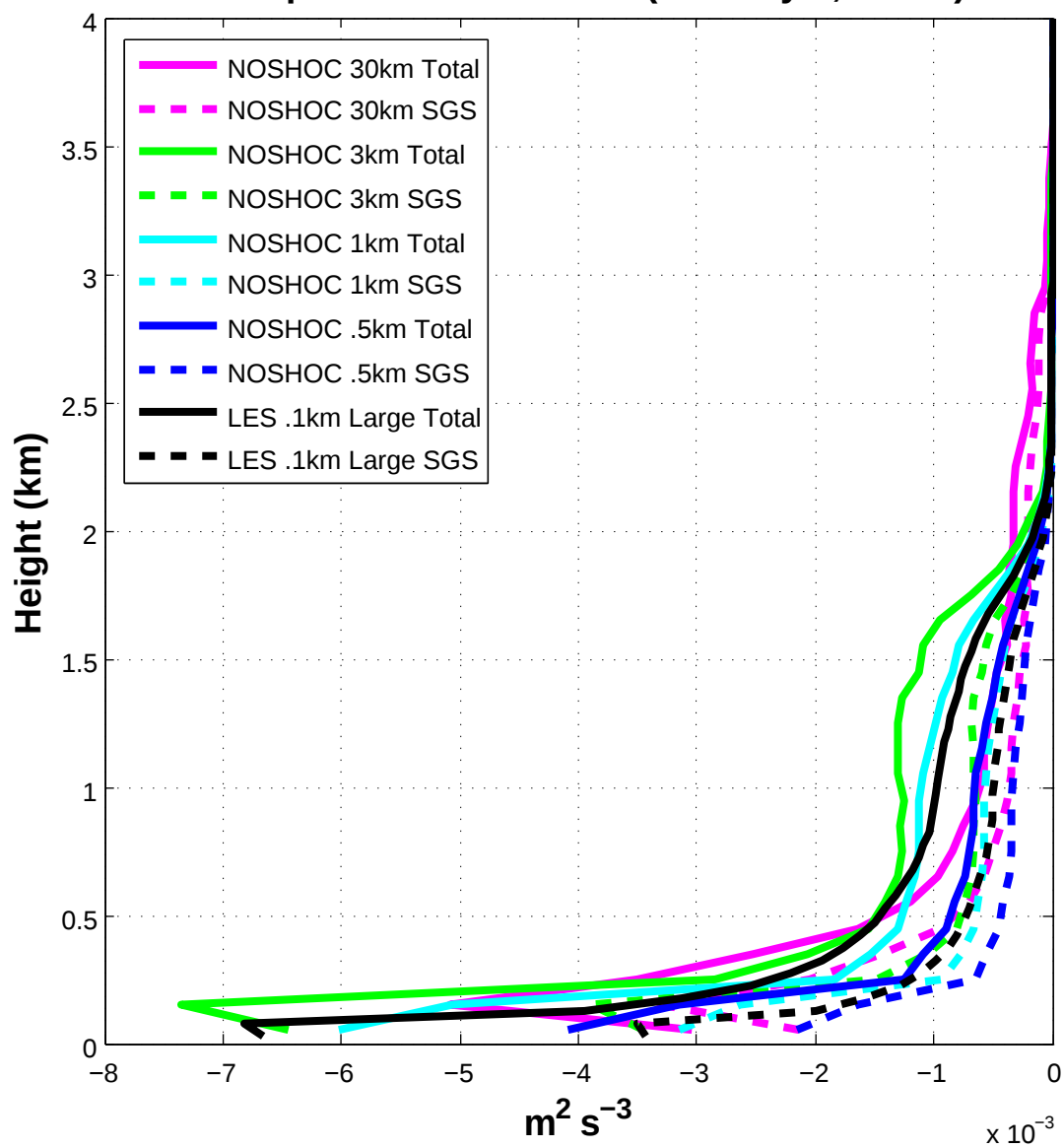
Dissipation terms of TKE (Full Phys., norad)
