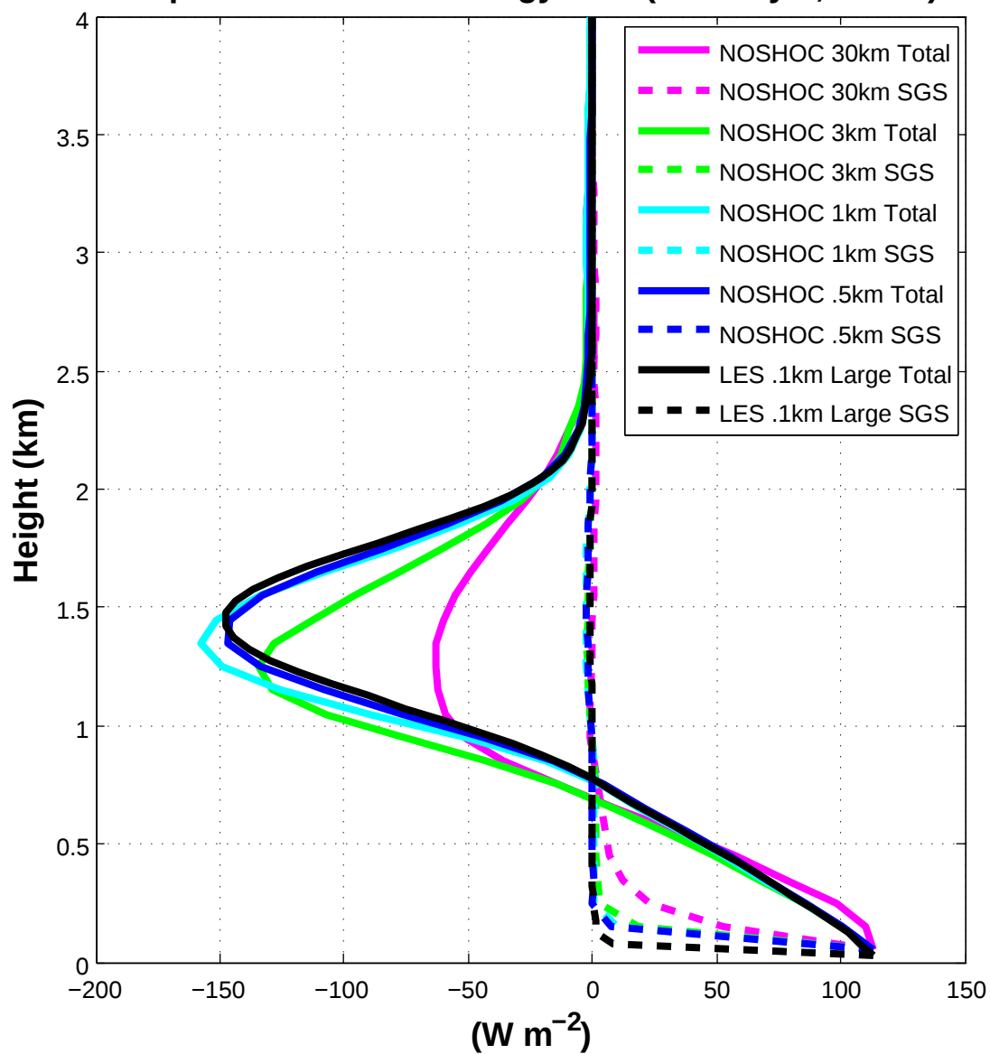
Liquid Water Static Energy Flux (Full Phys., norad)
