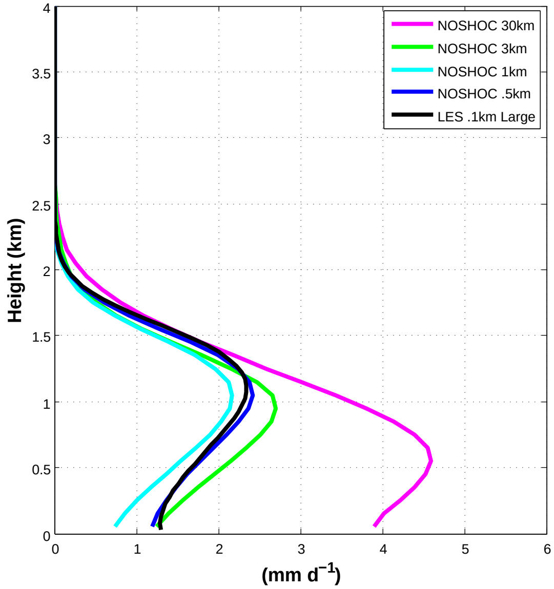
Precipitation Flux (Full Phys., norad)
