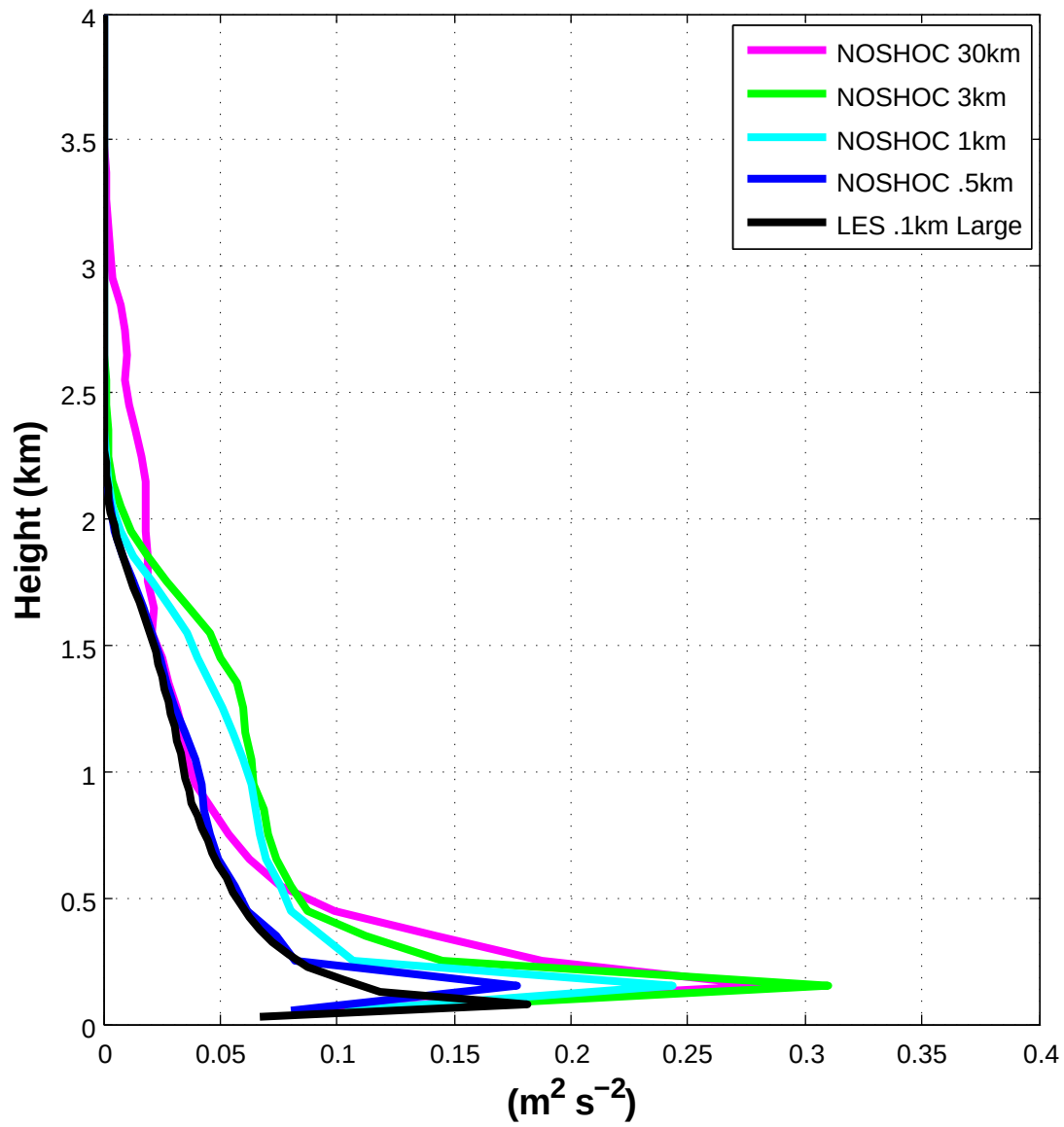
SGS Turbulent Kinetic Energy (Full Phys., norad)
