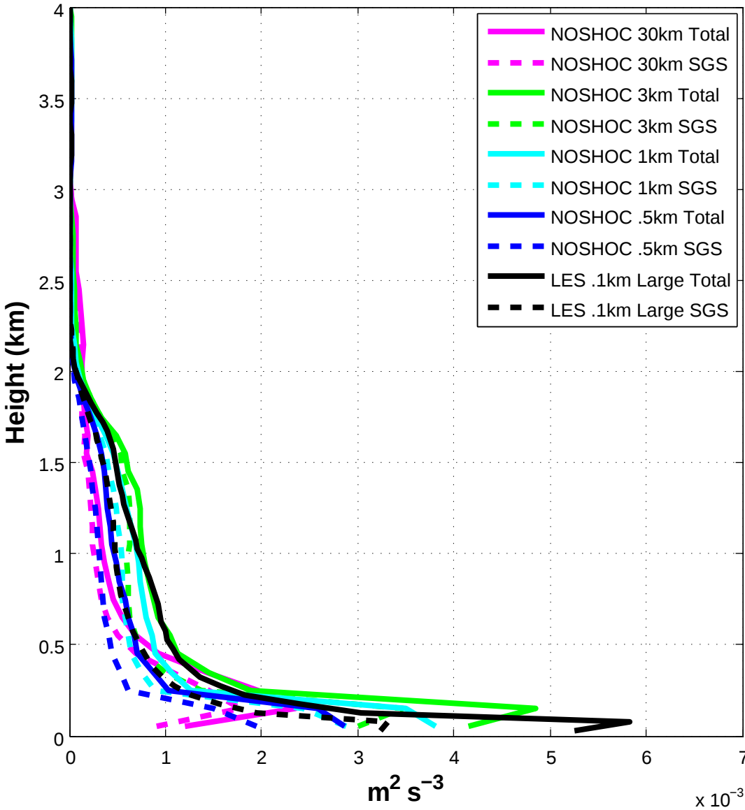
Shear production terms of TKE (Full Phys., norad)
