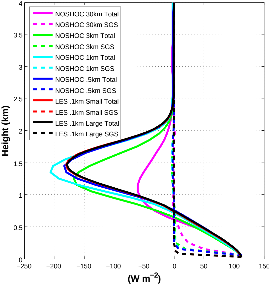
Liquid Water Static Energy Flux (Full Phys.)
