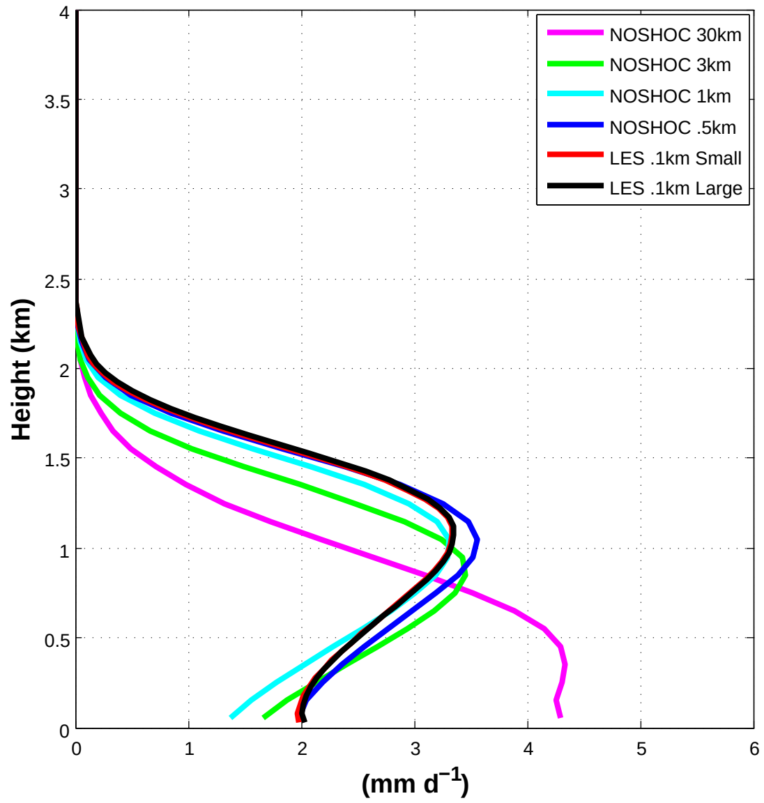
Precipitation Flux (Full Phys.)
