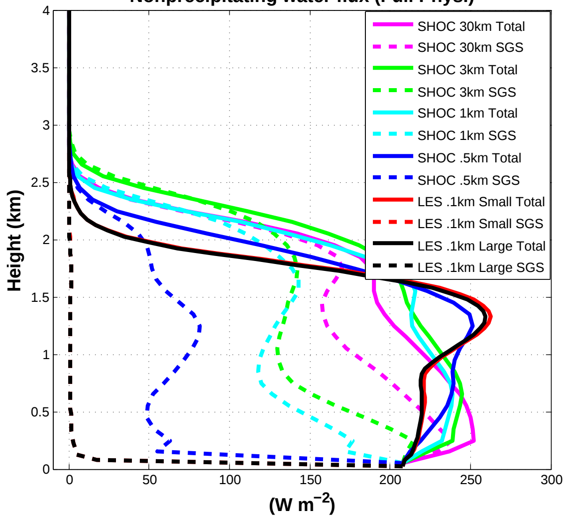
Nonprecipitating water flux (Full Phys.)
