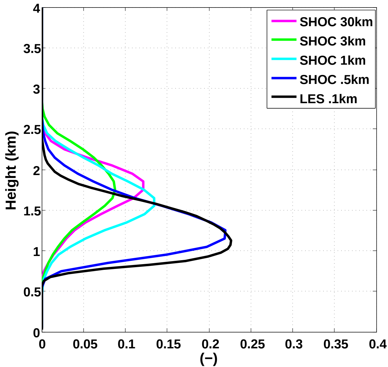
Cloud Fraction (Full Phys.)
