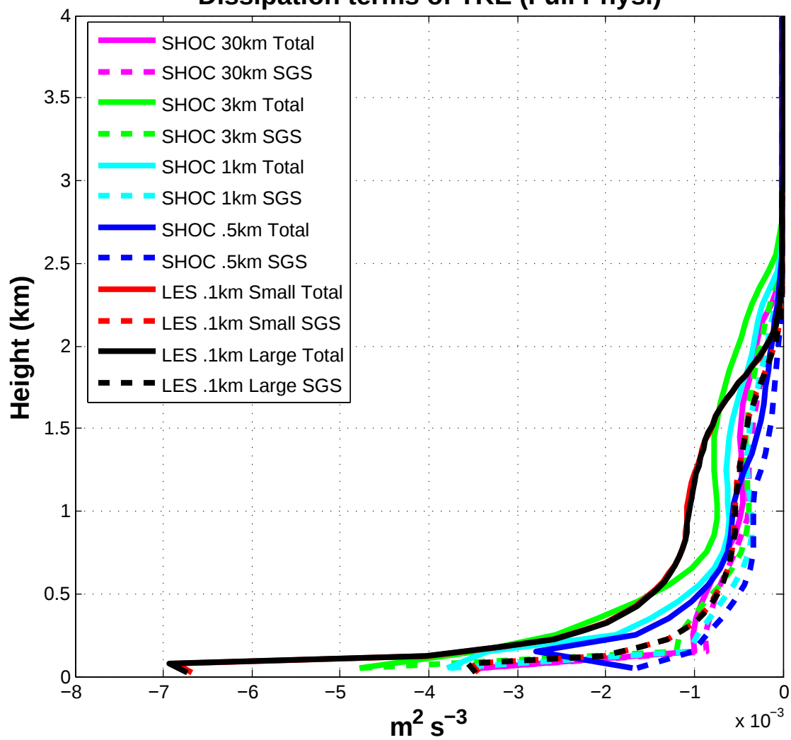
Dissipation terms of TKE (Full Phys.)
