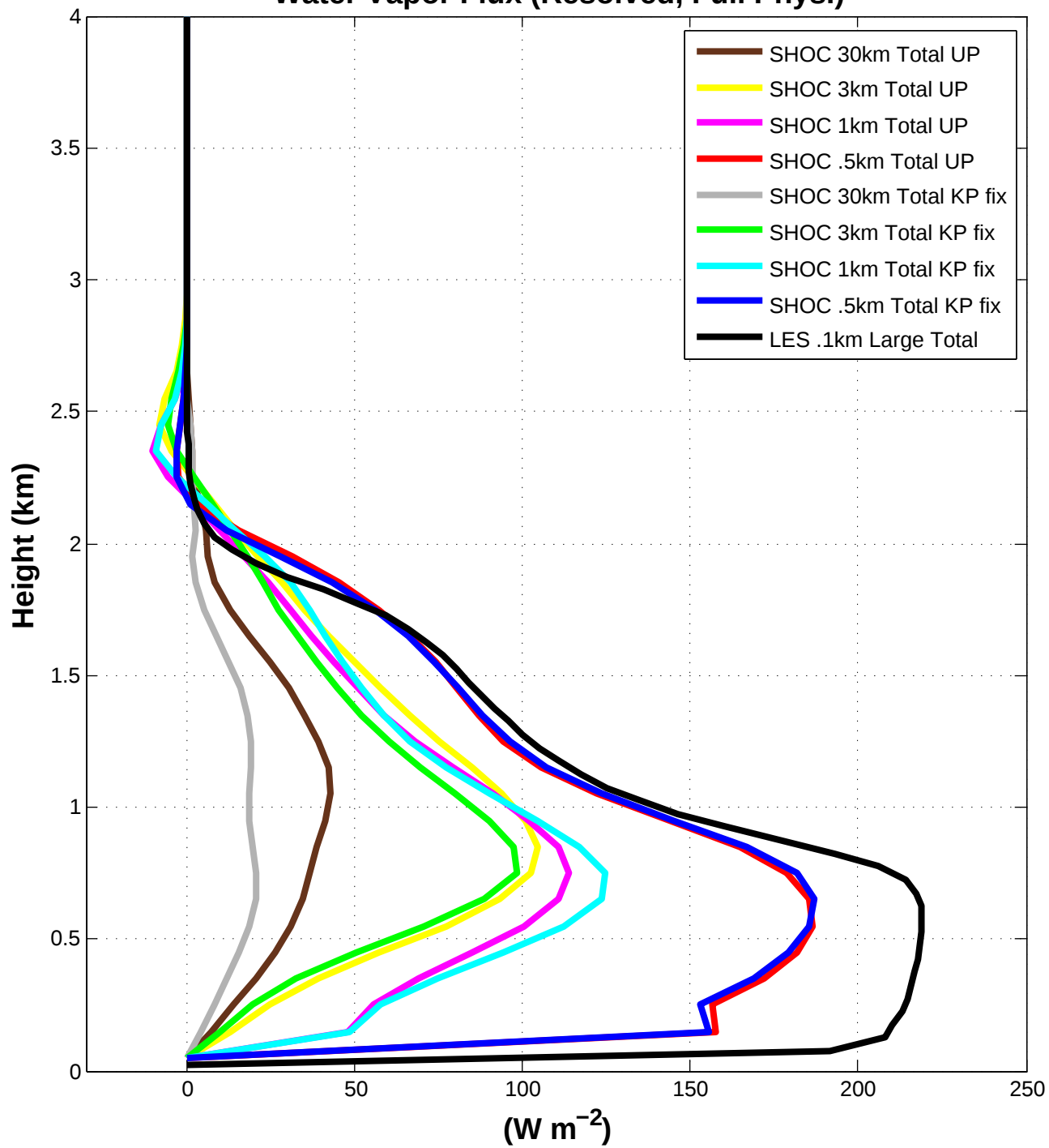
Water Vapor Flux (Resolved, Full Phys.)
