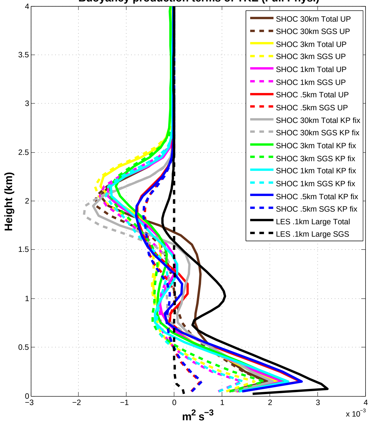
Buoyancy production terms of TKE (Full Phys.)
