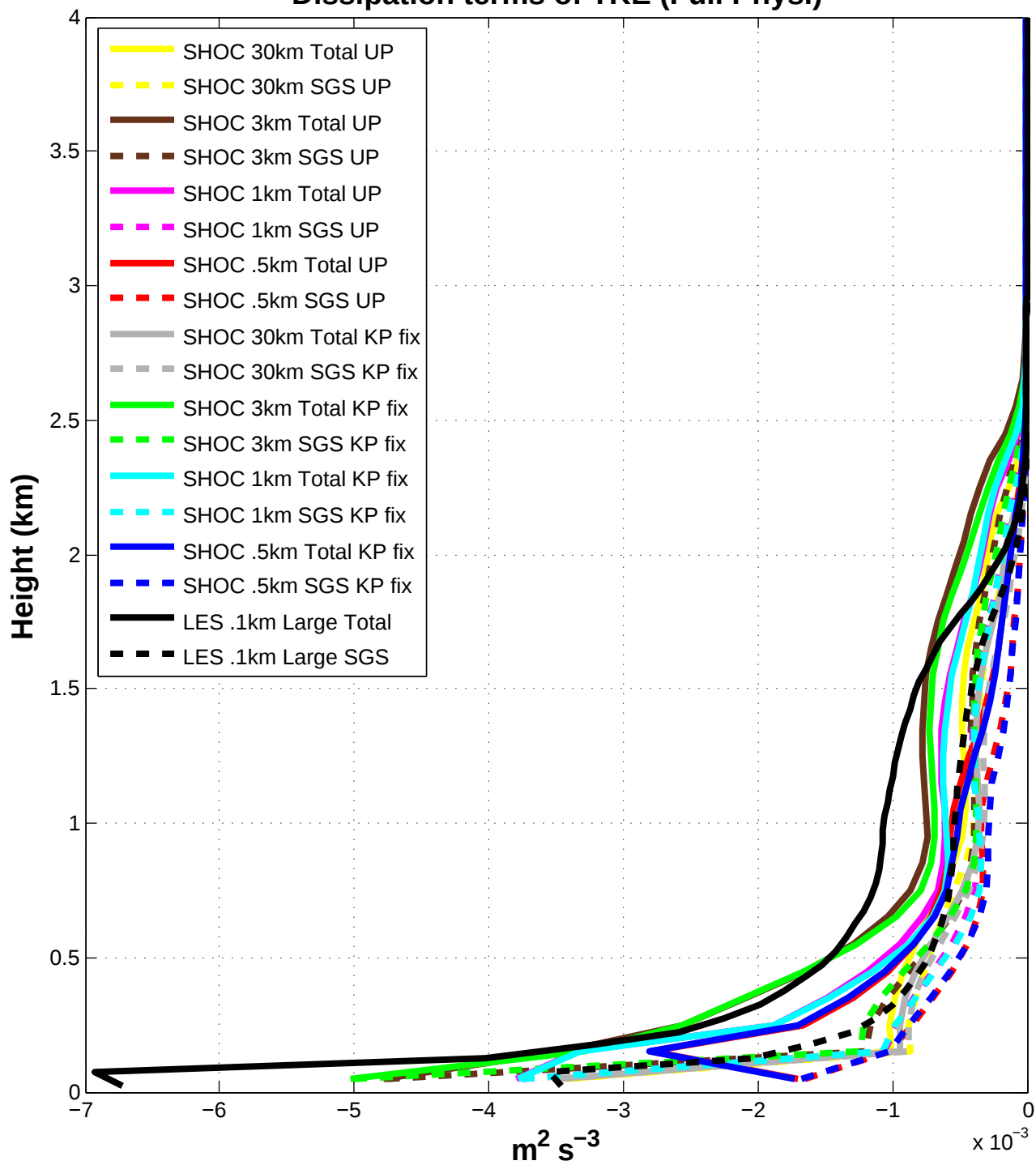
Dissipation terms of TKE (Full Phys.)
