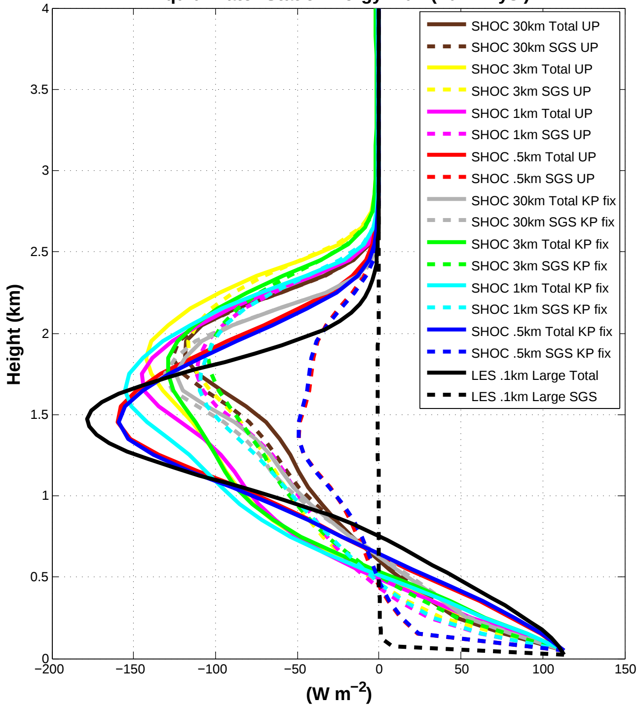
Liquid Water Static Energy Flux (Full Phys.)
