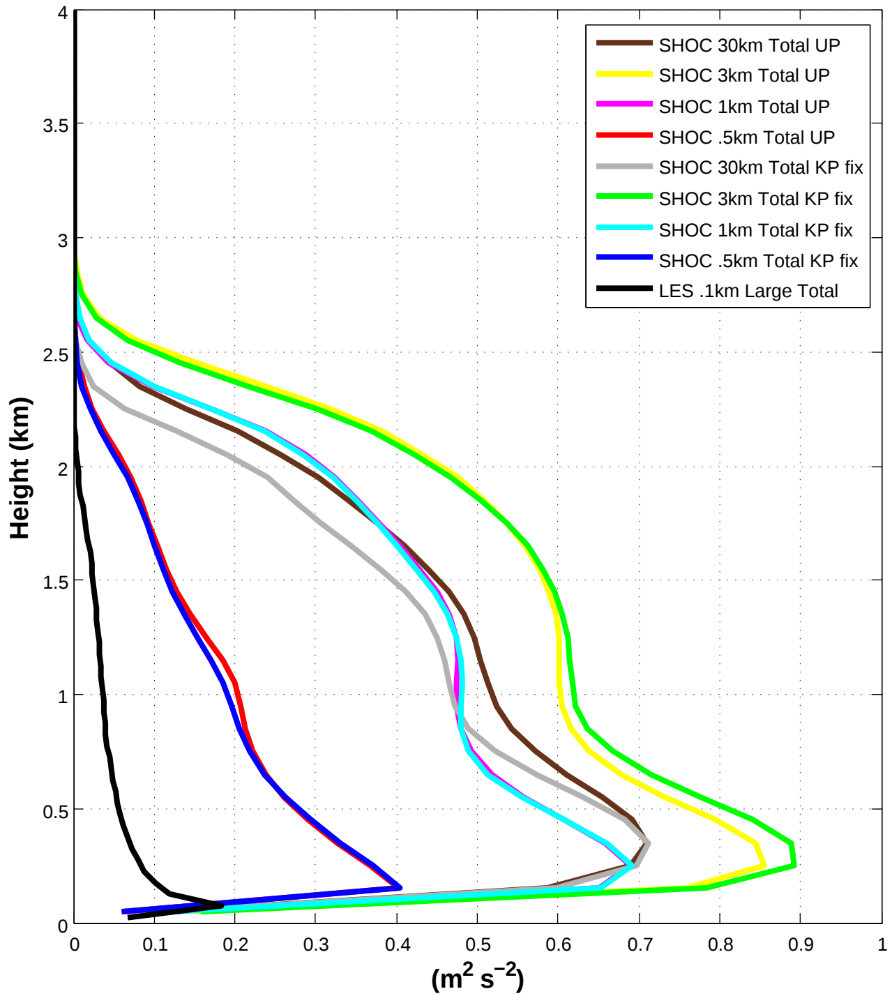
SGS Turbulent Kinetic Energy (Full Phys.)
