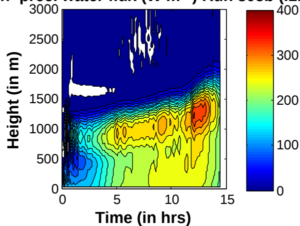
Non-prec. water flux ( \text{W m}^{-2} ) Run 805b (.1km)
