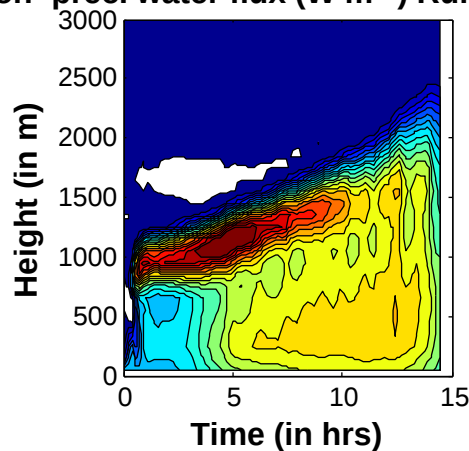
Non-prec. water flux ( \text{W m}^{-2} ) Run 805b (.1km)
