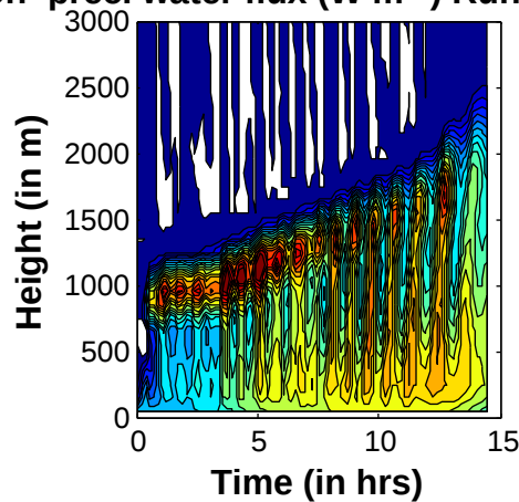
Non-prec. water flux ( \text{W m}^{-2} ) Run 602 (1km) Non-prec. water flux ( \text{W m}^{-2} ) Run 603 (.5km)
