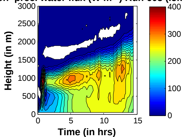
Non-prec. water flux ( \text{W m}^{-2} ) Run 602 (1km) Non-prec. water flux ( \text{W m}^{-2} ) Run 603 (.5km)
