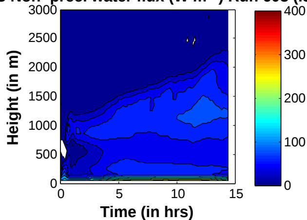
SGS Non-prec. water flux ( \text{W m}^{-2} ) Run 602 (1km)
