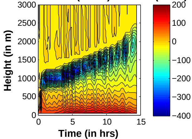
Total LWSE flux ( \text{W m}^{-2} ) Run 602 (1km)
