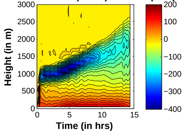
Total LWSE flux ( \text{W m}^{-2} ) Run 603 (.5km)
