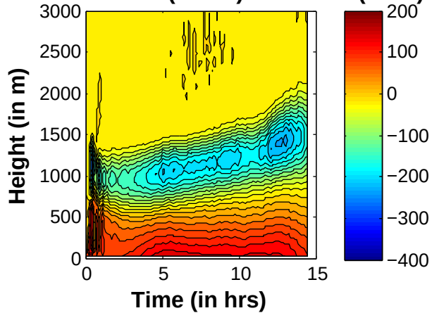
Total LWSE flux ( \text{W m}^{-2} ) Run 805b (.1km)
