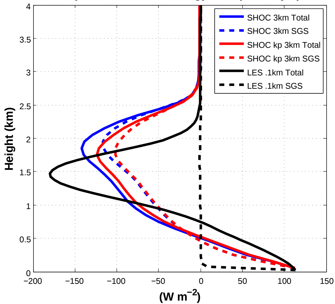
Liquid Water Static Energy Flux (Full Phys.)
