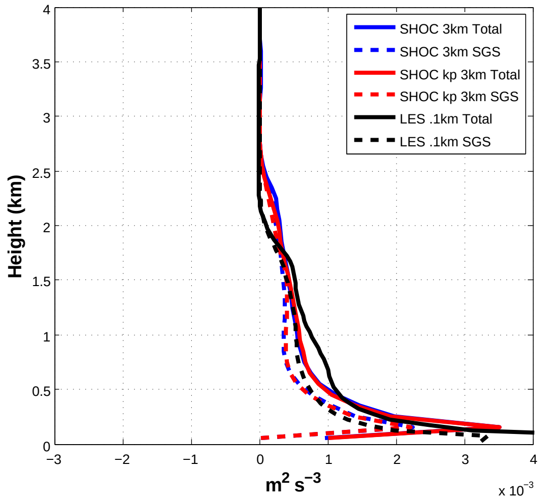
Shear production terms of TKE (Full Phys.)
