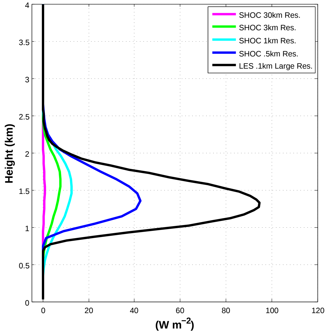
Liquid Water Flux (Full Phys., norad)
