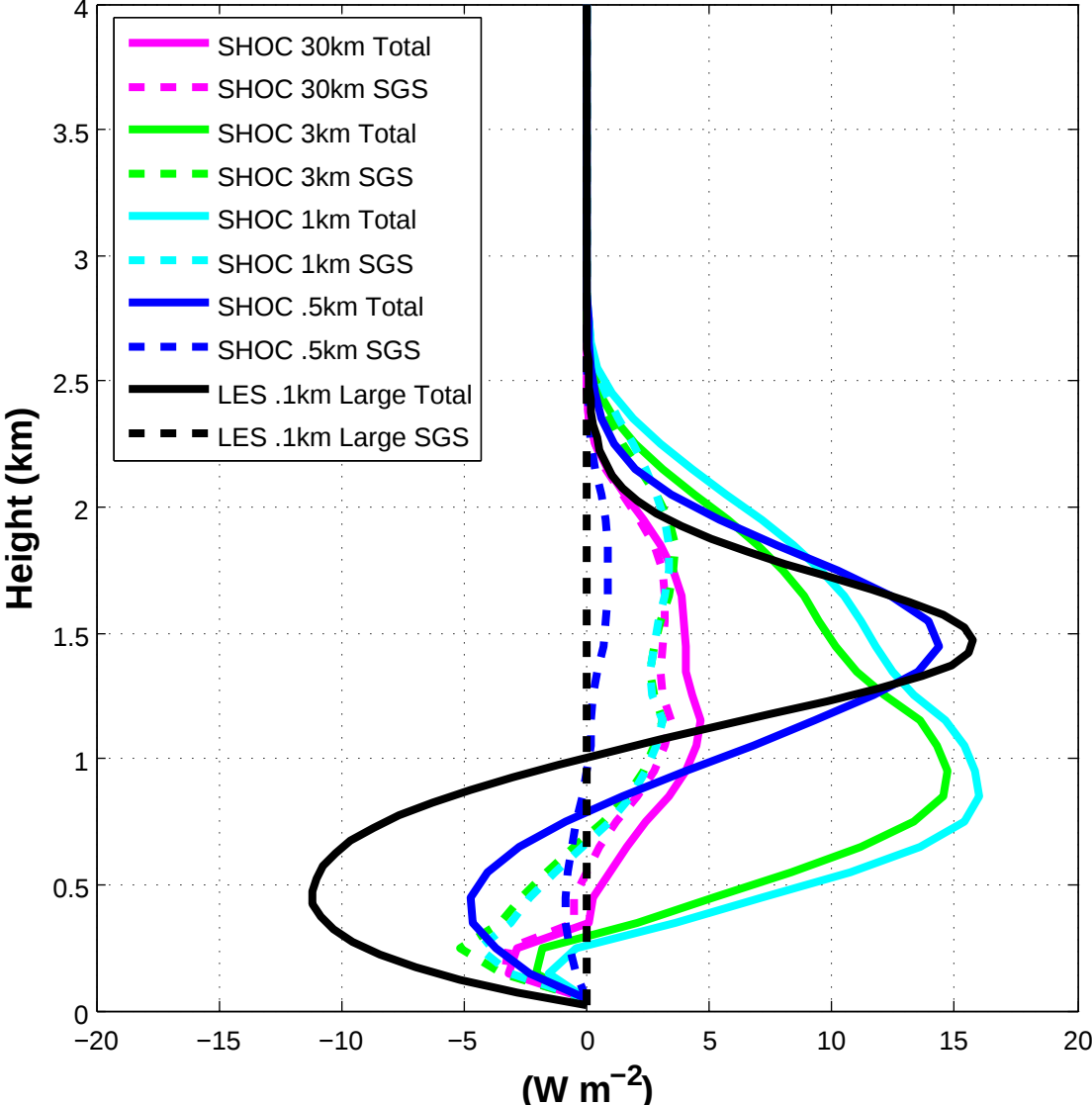
Precipitating-water turbulent flux (Full Phys., norad)
