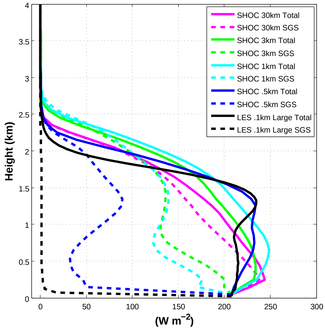
Nonprecipitating water flux (Full Phys., norad)
