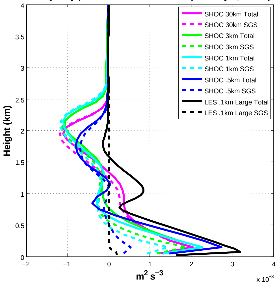
Buoyancy production terms of TKE (Full Phys., norad)
