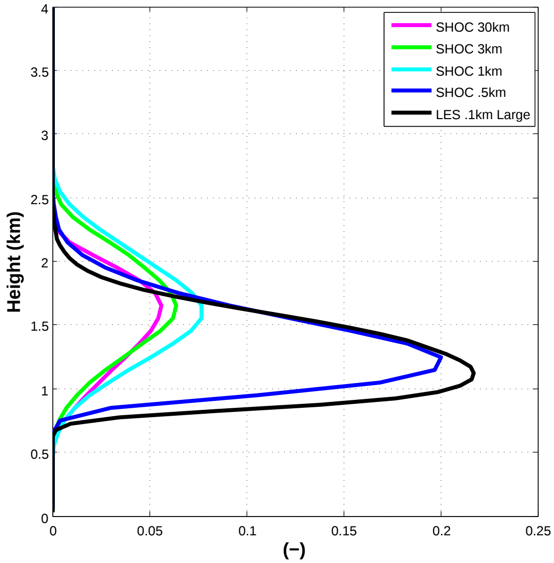
Cloud Fraction (Full Phys., norad)
