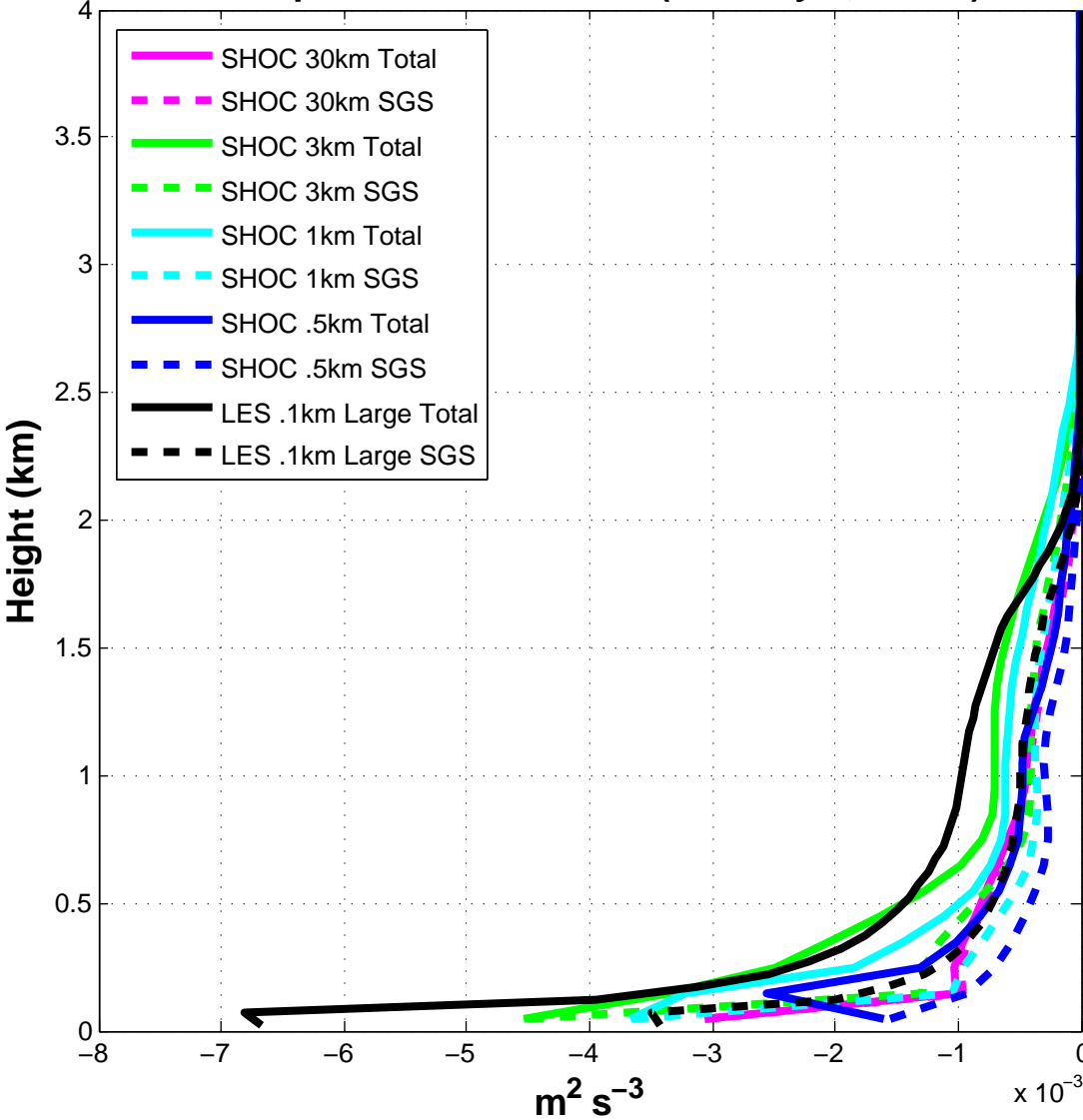
Dissipation terms of TKE (Full Phys., norad)
