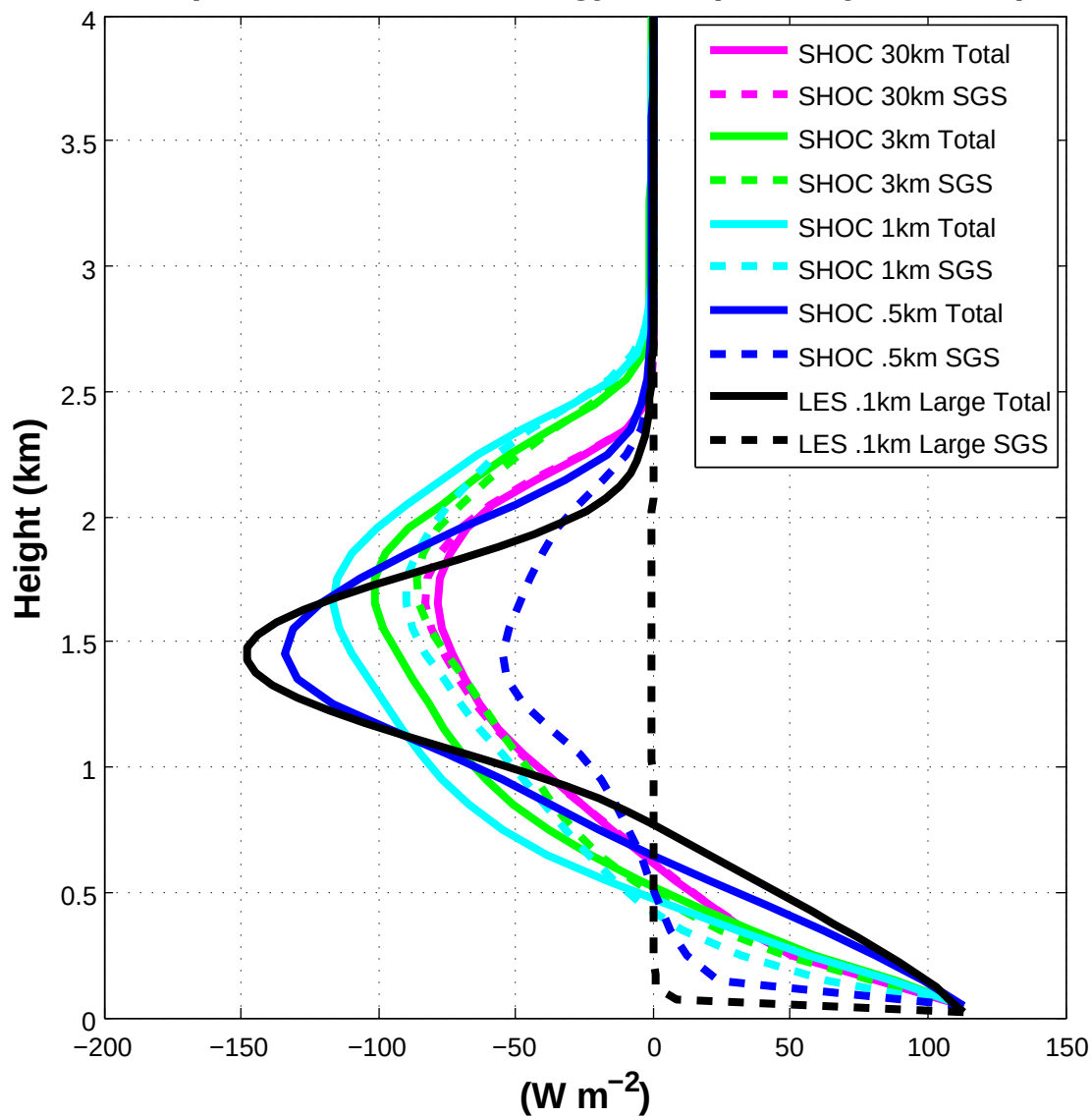
Liquid Water Static Energy Flux (Full Phys., norad)
