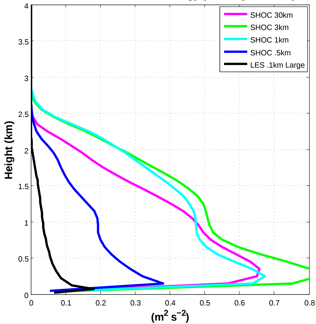
SGS Turbulent Kinetic Energy (Full Phys., norad)
