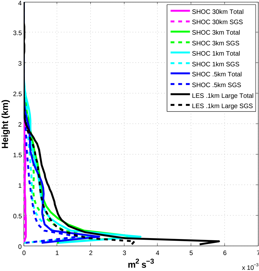
Shear production terms of TKE (Full Phys., norad)
