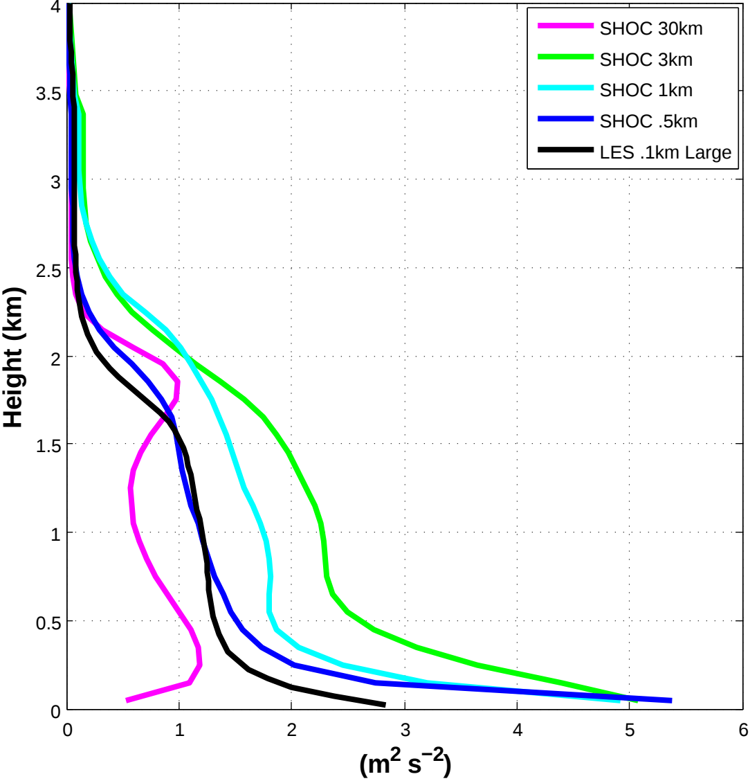
Total Turbulent Kinetic Energy (Full Phys., norad)
