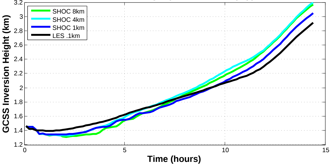
Inversion Height (Ice, no rad/sed/pcp)
