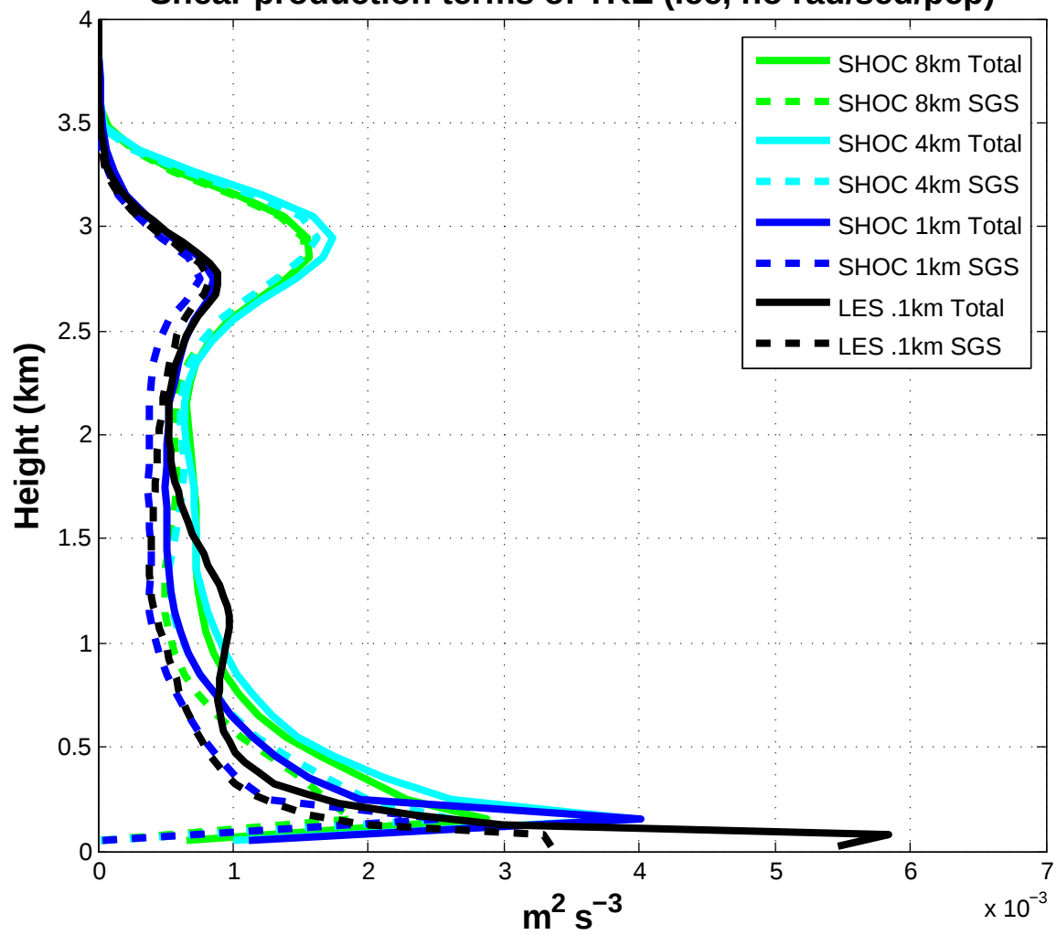
Shear production terms of TKE (Ice, no rad/sed/pcp)
