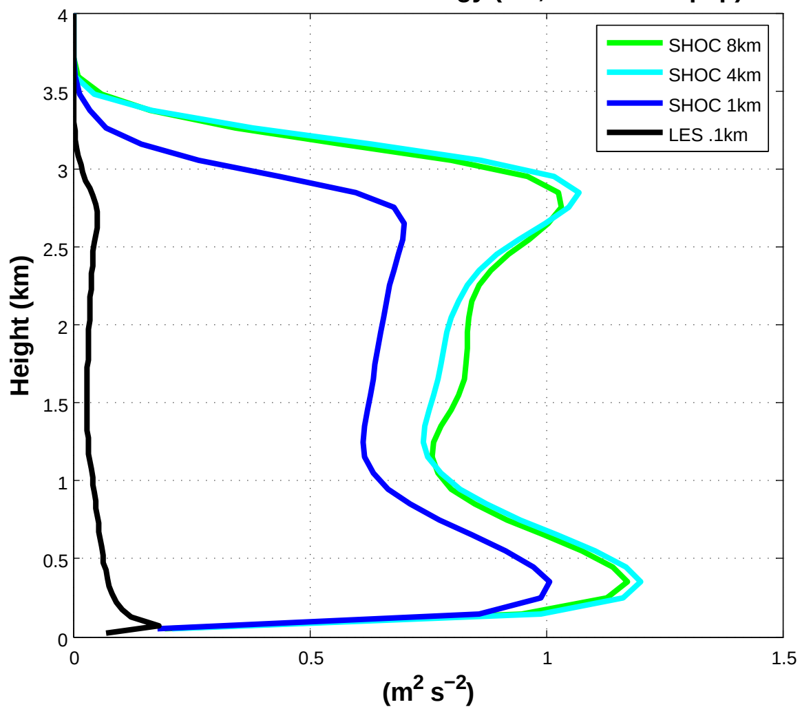
SGS Turbulent Kinetic Energy (ice, no rad/sed/pcp)
