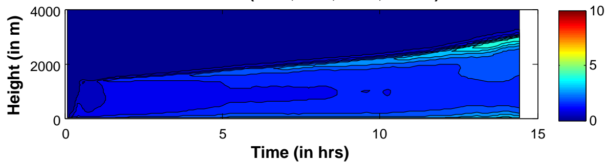
TKE Total (805c, LES, .1km, no ice)
