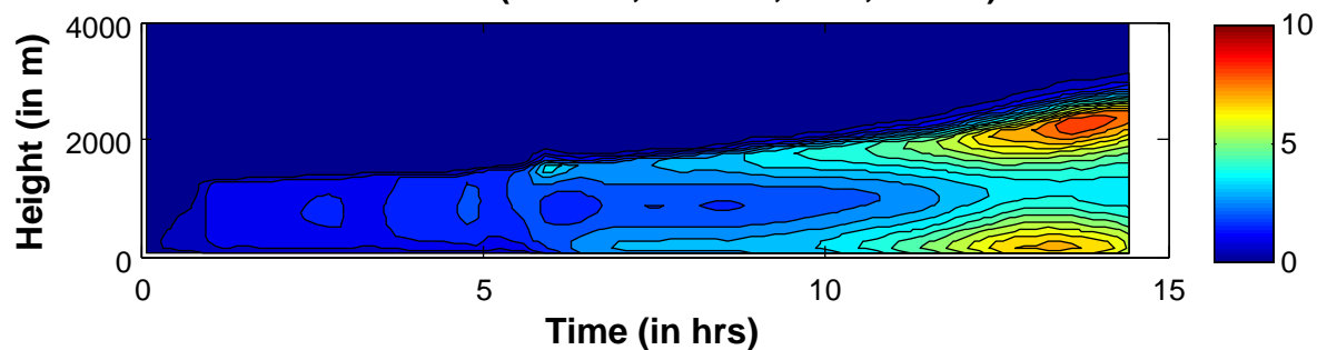
TKE Total (602c-h, .5x-mix, 1km, no ice)
