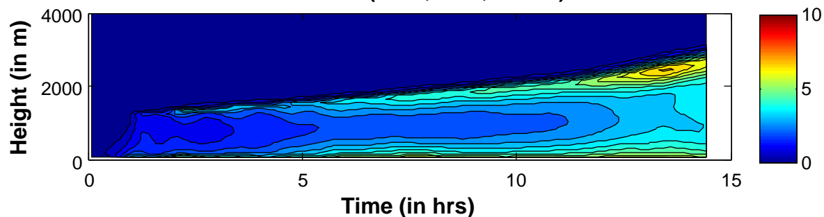
TKE Total (602c-d, 2x-mix, 1km, no ice)
