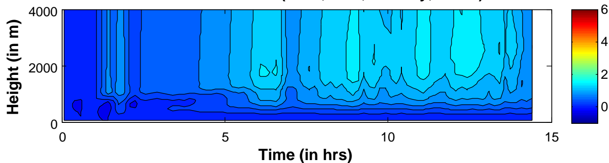
Conv. Vel. Scale W^3 (602d, 1km, ice only, m^3 s^{-3} )
