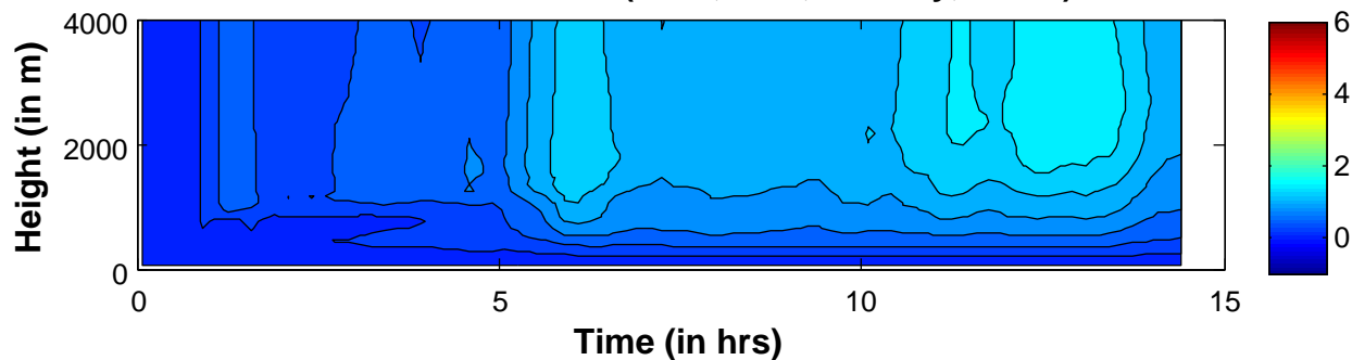
Conv. Vel. Scale W^3 (603d, .5km, ice only, m^3 s^{-3} )
