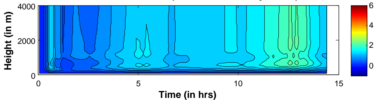
Conv. Vel. Scale W^3 (805d, .1km, ice only, m^3 s^{-3} )
