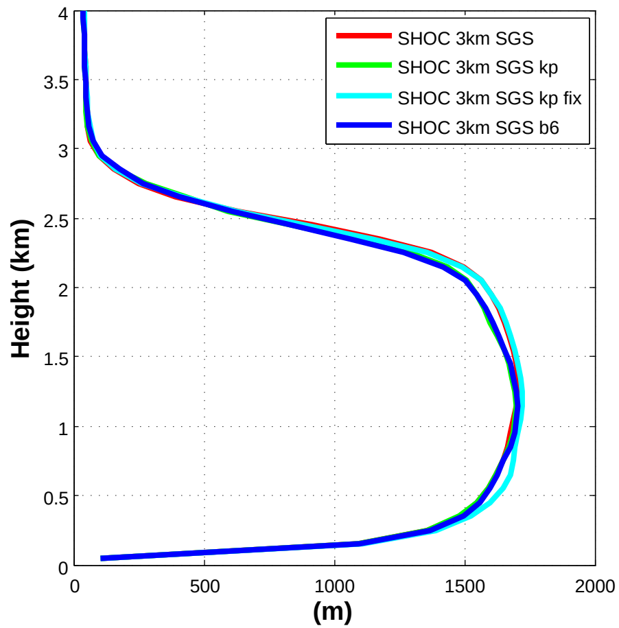
SGS Mixing Length (full phys)
