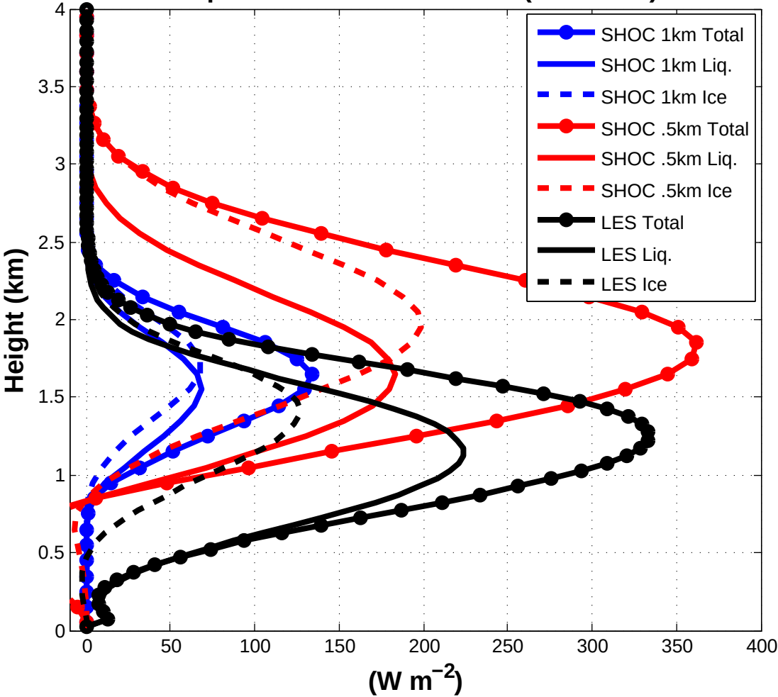
Liquid Water and Cloud Ice (Resolved)
