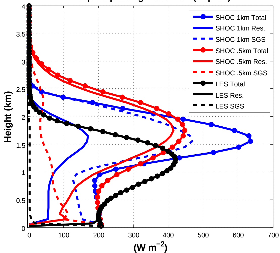
Nonprecipitating water flux (noprec)
