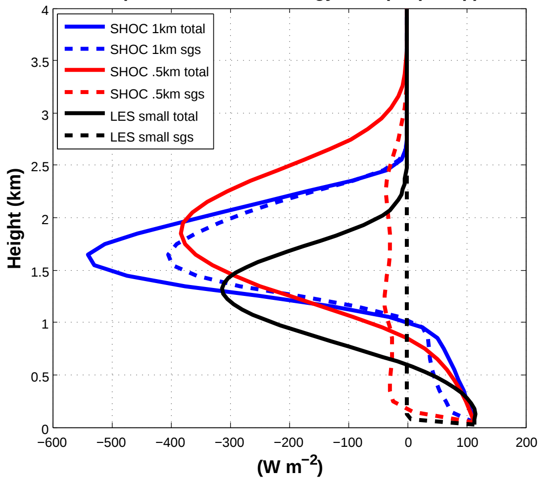
Liquid Water Static Energy Flux (no precip)
