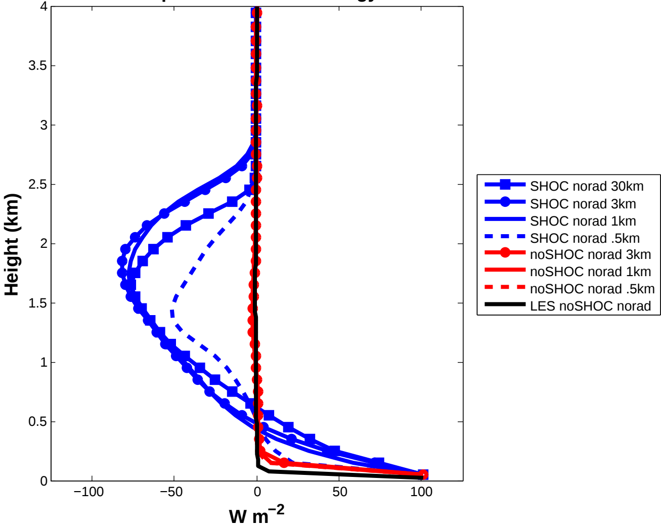
SGS Liquid Water Static Energy Flux
