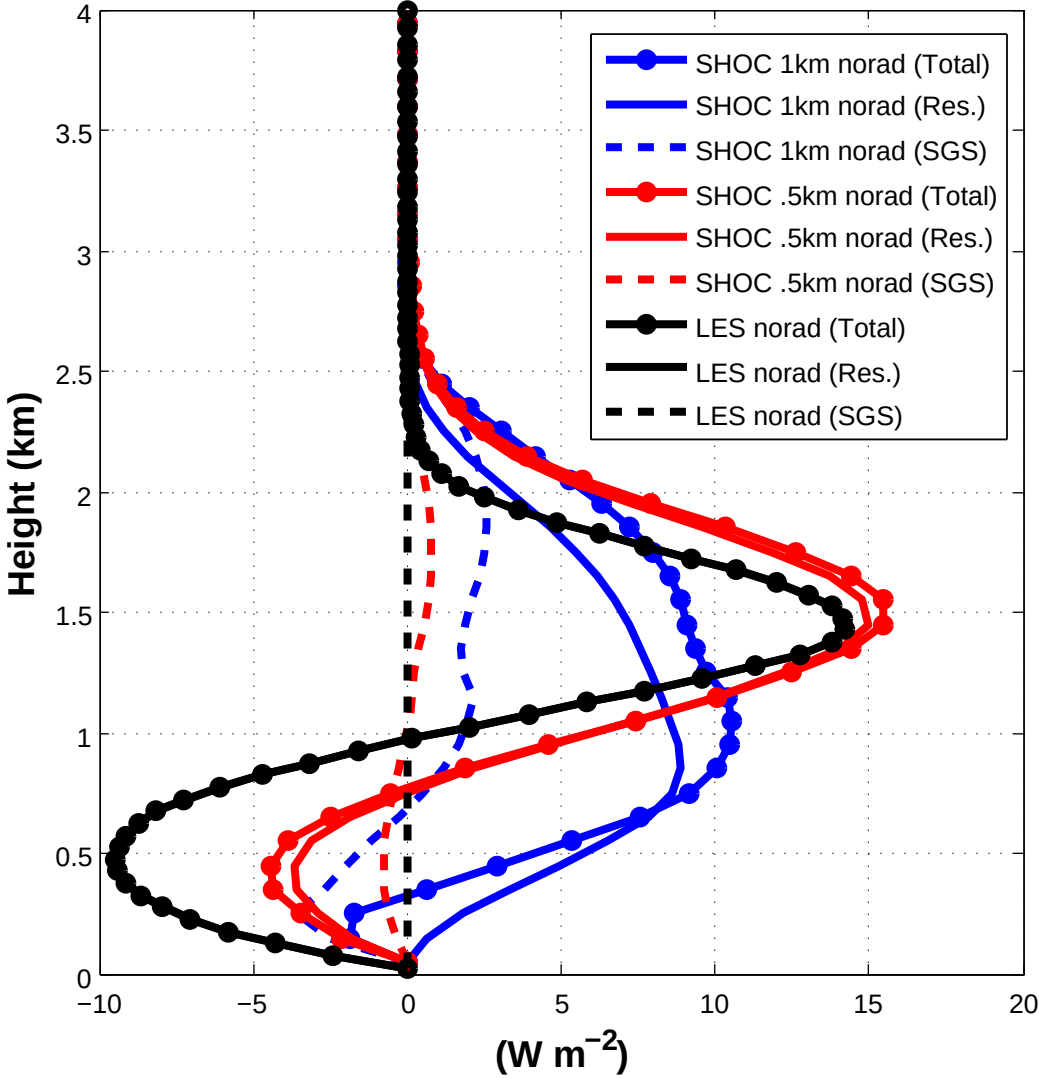
Precipitating-water turbulent flux
